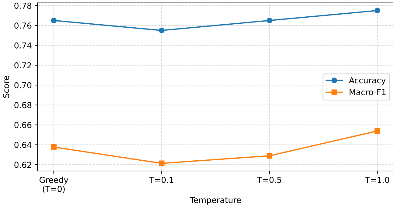
Qwen2.5-1.5B - Temperature vs Performance
